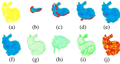
Figure 6: Surface reconstruction from the point cloud dataset of the Stanford bunny.
